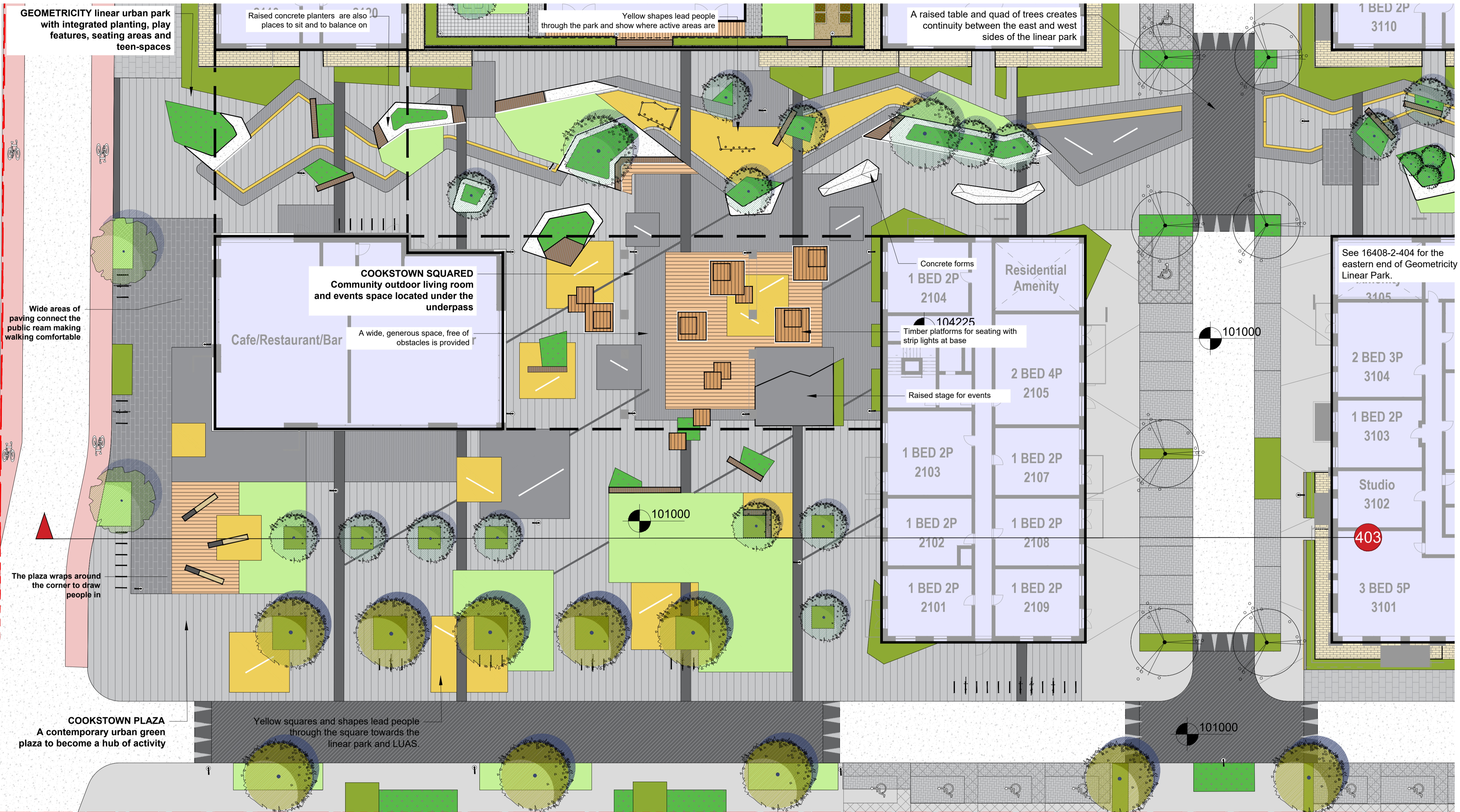
Block B underpass & plaza plan - scale 1:200
